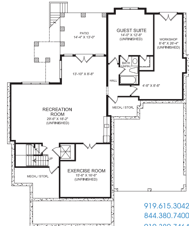
BASEMENT
